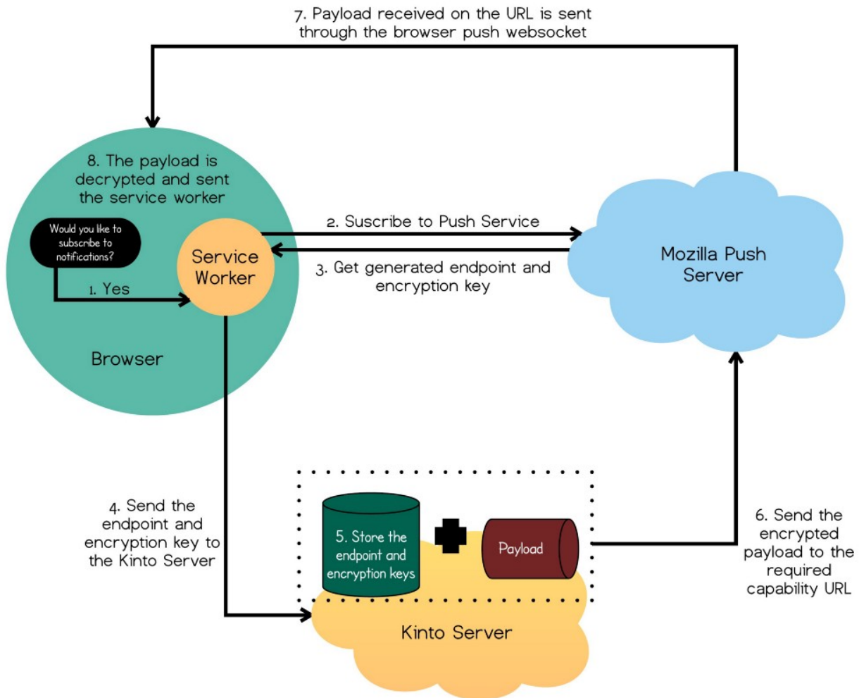
Fig. 1.1: Example of how we could use WebPush with Kinto.
